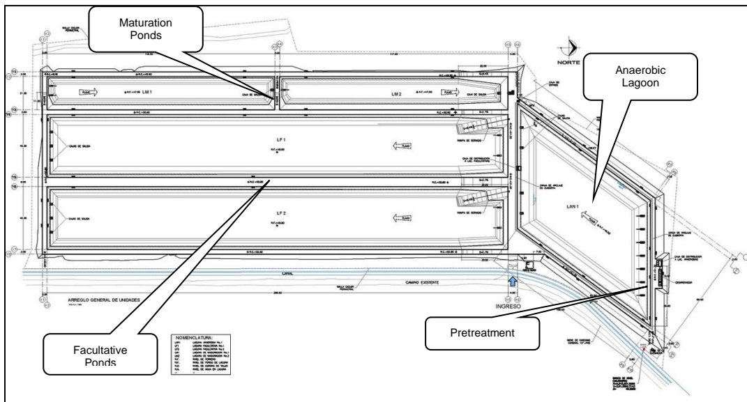
Figure 4 GENERAL LAYOUT OF THE WASTEWATER TREATMENT PLANT
