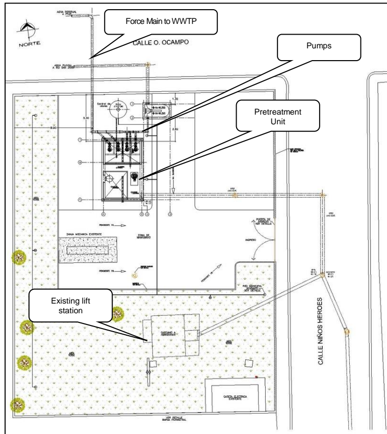
Figure 3 GENERAL LAYOUT OF THE MAIN LIFT STATION
